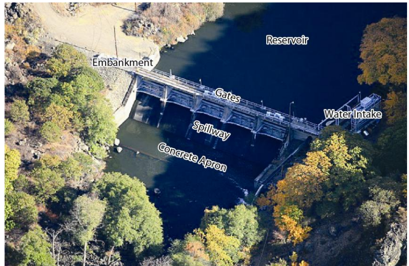
Figure 4.2-8: Photo of Copco 2 Dam and Reservoir with Specific Components Labeled. With full facilities removal, all visible components would be removed. With partial facilities removal, certain components (e.g., penstock) would be retained.
