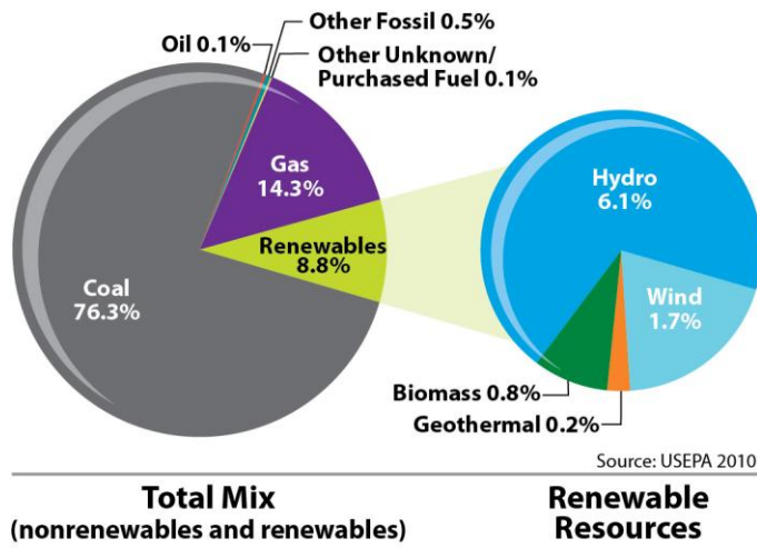
Figure 4.4.11-1: PacifiCorp Power Control Area Generation Resource Mix (as of 2007)
