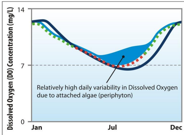
Figure 4.1-21: With dam removal, dissolved oxygen in the Klamath River downstream of Iron Gate Dam would consistently achieve North Coast Basin Plan percent saturation objectives and would be greater than dissolved oxygen under existing conditions from April through November. Dam removal may also result in greater variability in dissolved oxygen during June through October due to photosynthesis and respiration of attached algae (periphyton) that establish in the free-flowing river. Lines represent simplified TMDL model output of hourly values from NCRWQCB.
